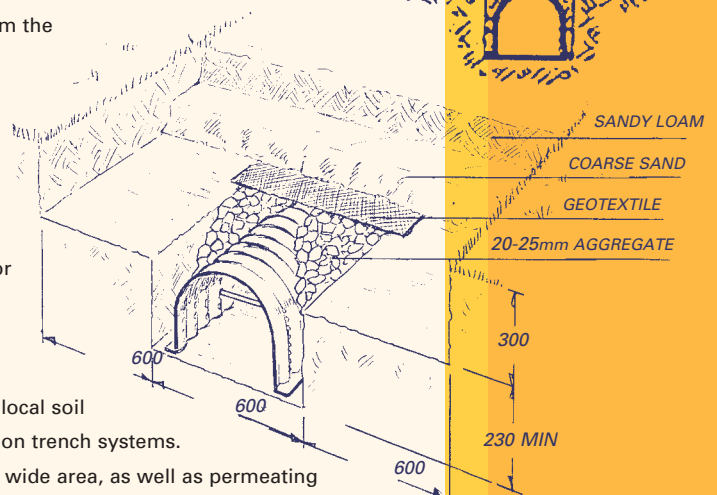
METHOD 2: Transpiration Trenches and Beds
